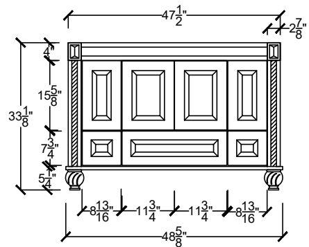
ANAV 4822 BD- - - - CENTER BOWL SINK
