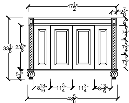
ANAV 4822 - - - - CENTER BOWL SINK
